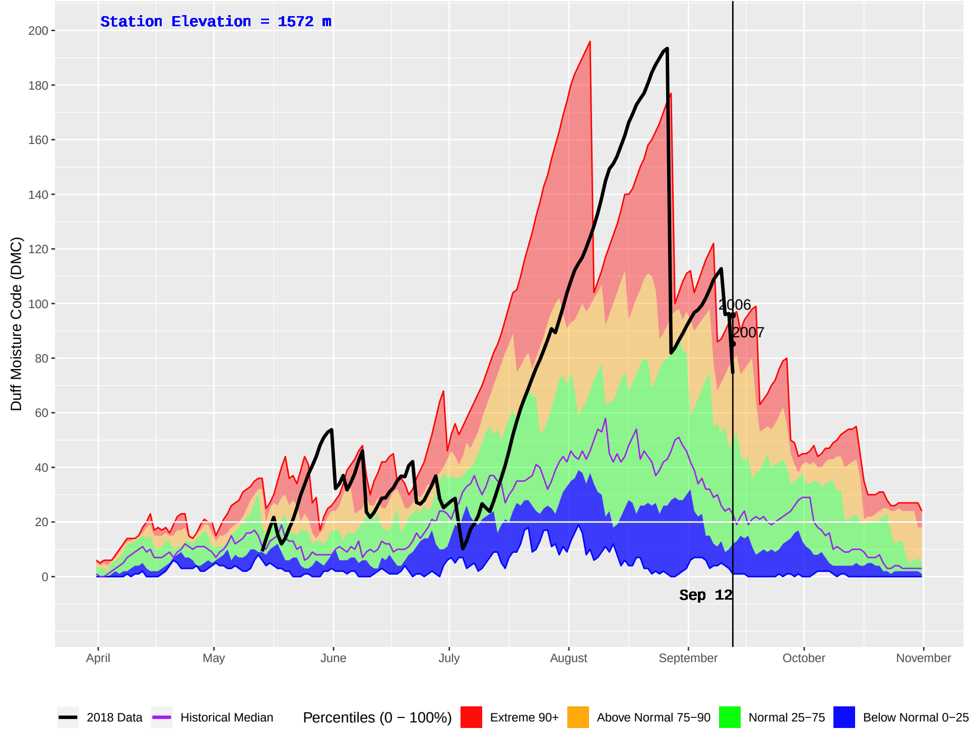
NEGRO CREEK (789) : Historical (2001–2016) and Current (2018) Daily Duff Moisture Code (DMC)
