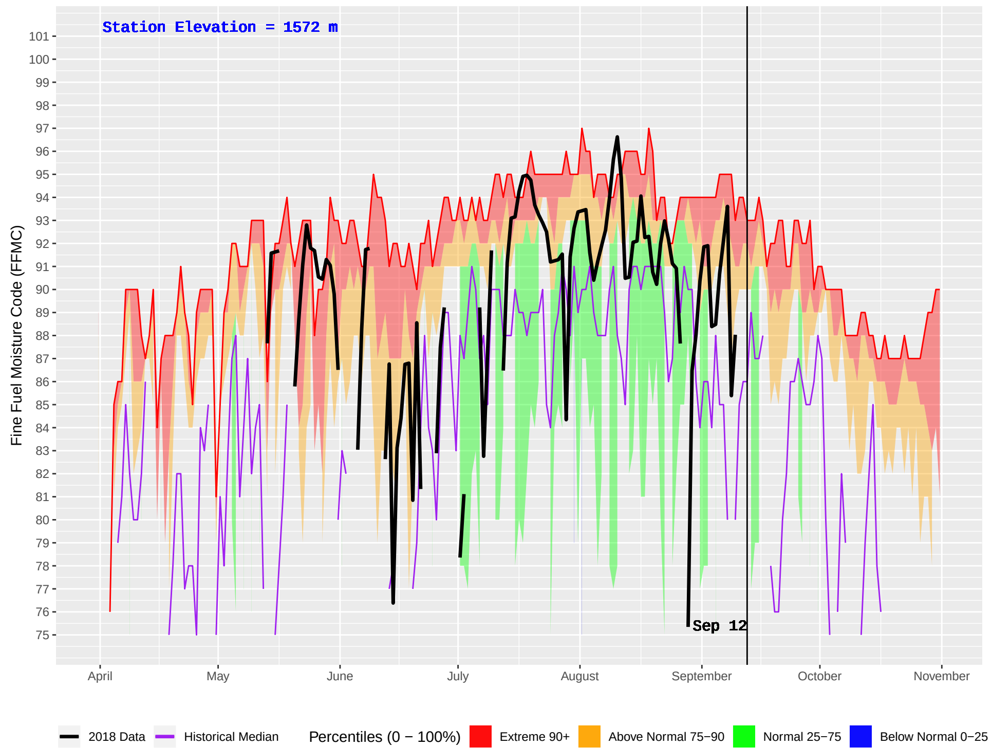
NEGRO CREEK (789) : Historical (2001–2016) and Current (2018) Daily Fine Fuel Moisture Code (FFMC)
