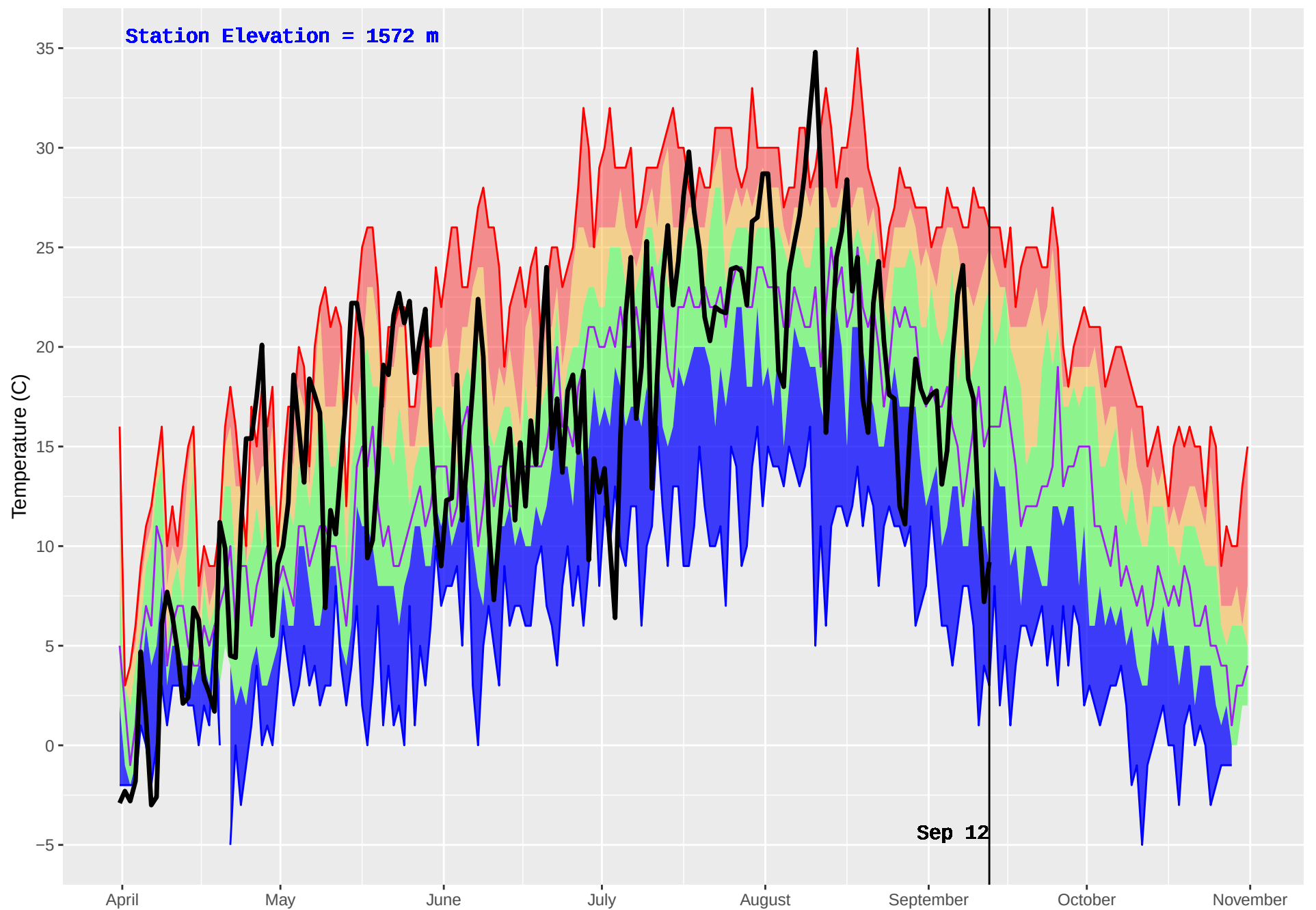
NEGRO CREEK (789) : Historical (2001–2016) and Current (2018) Daily Temperature
