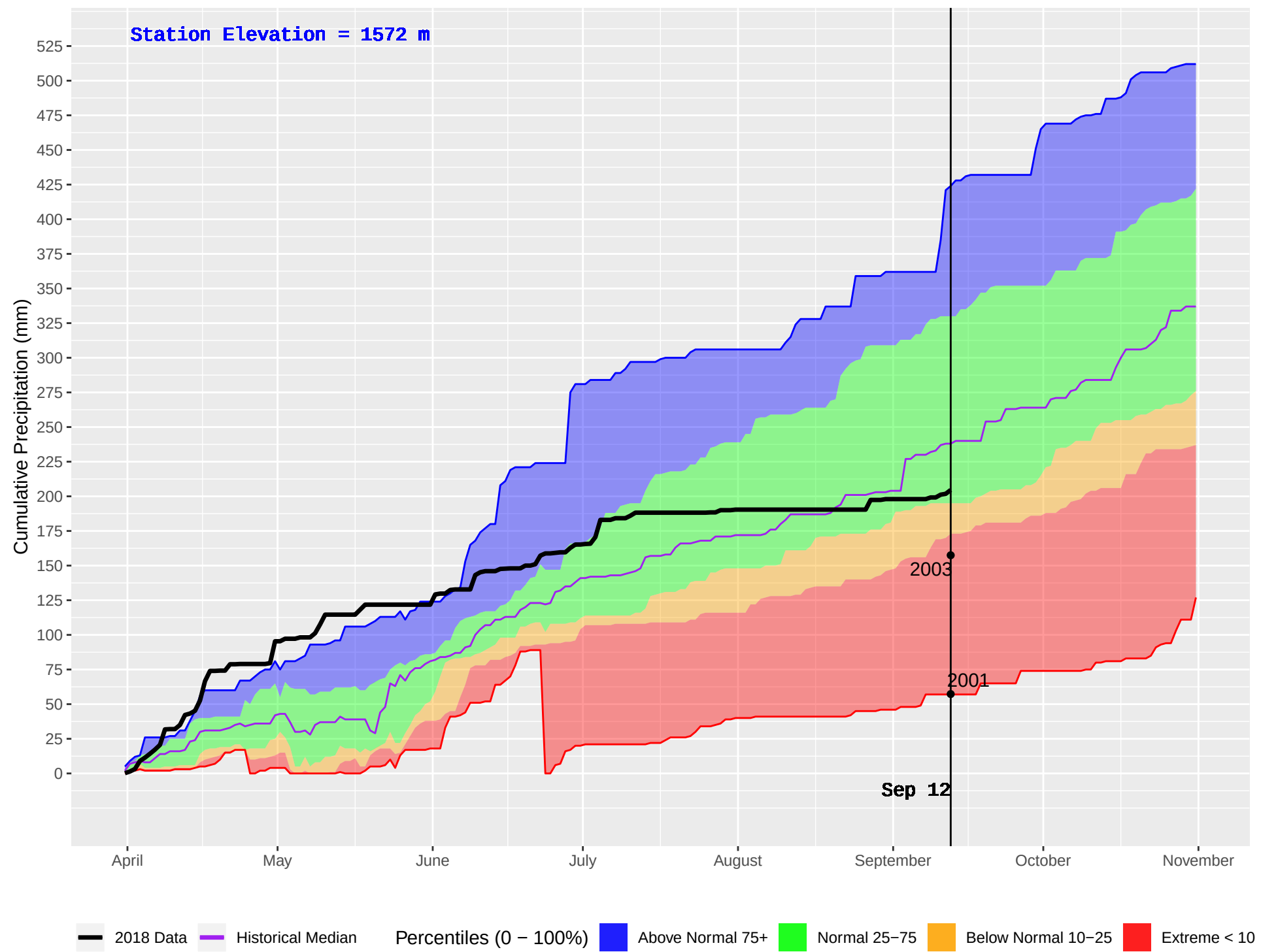
NEGRO CREEK (789) : Historical (2001–2016) and Current (2018) Daily Cumulative Precipitation
