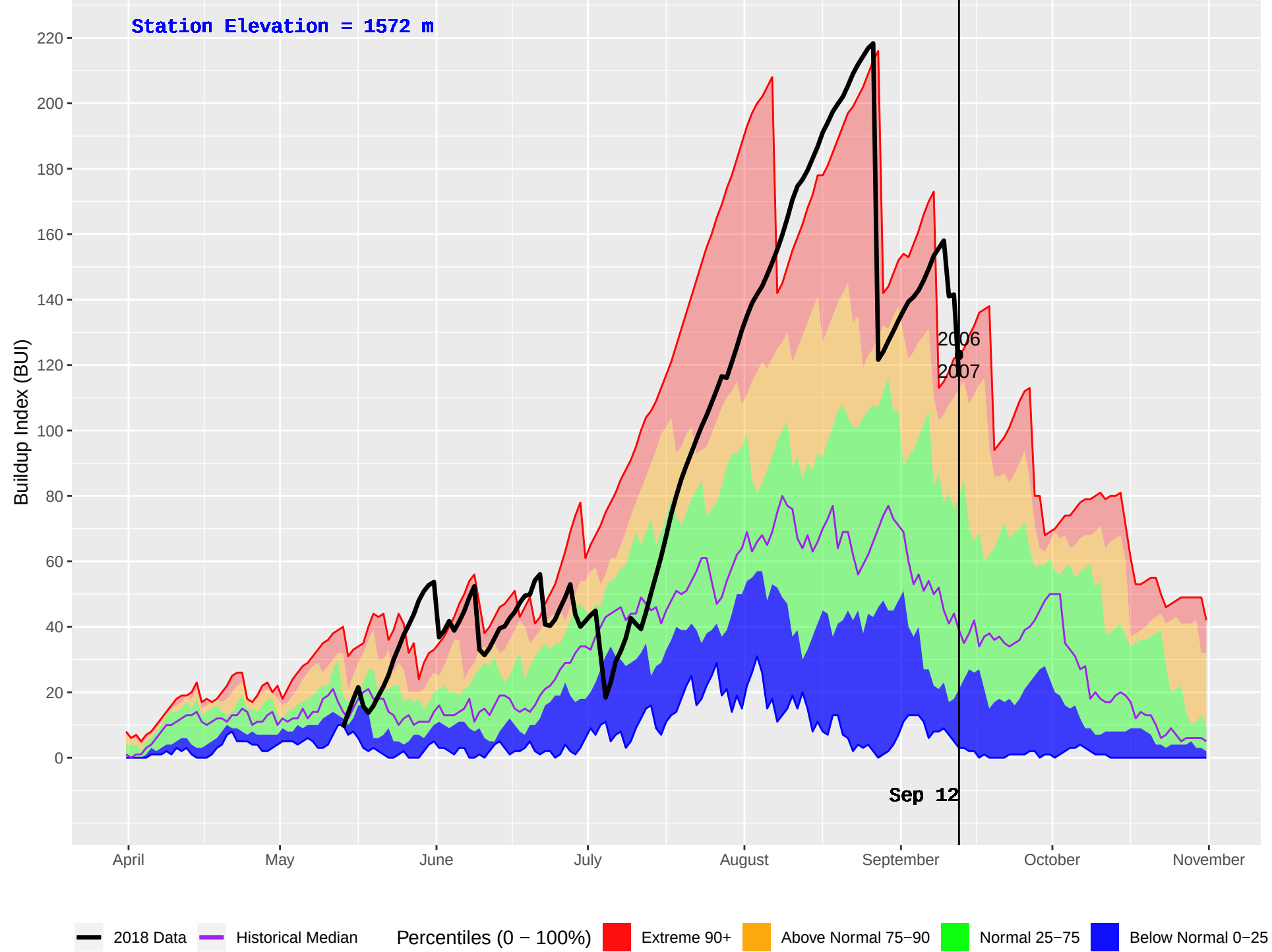
NEGRO CREEK (789) : Historical (2001–2016) and Current (2018) Daily Buildup Index (BUI)
