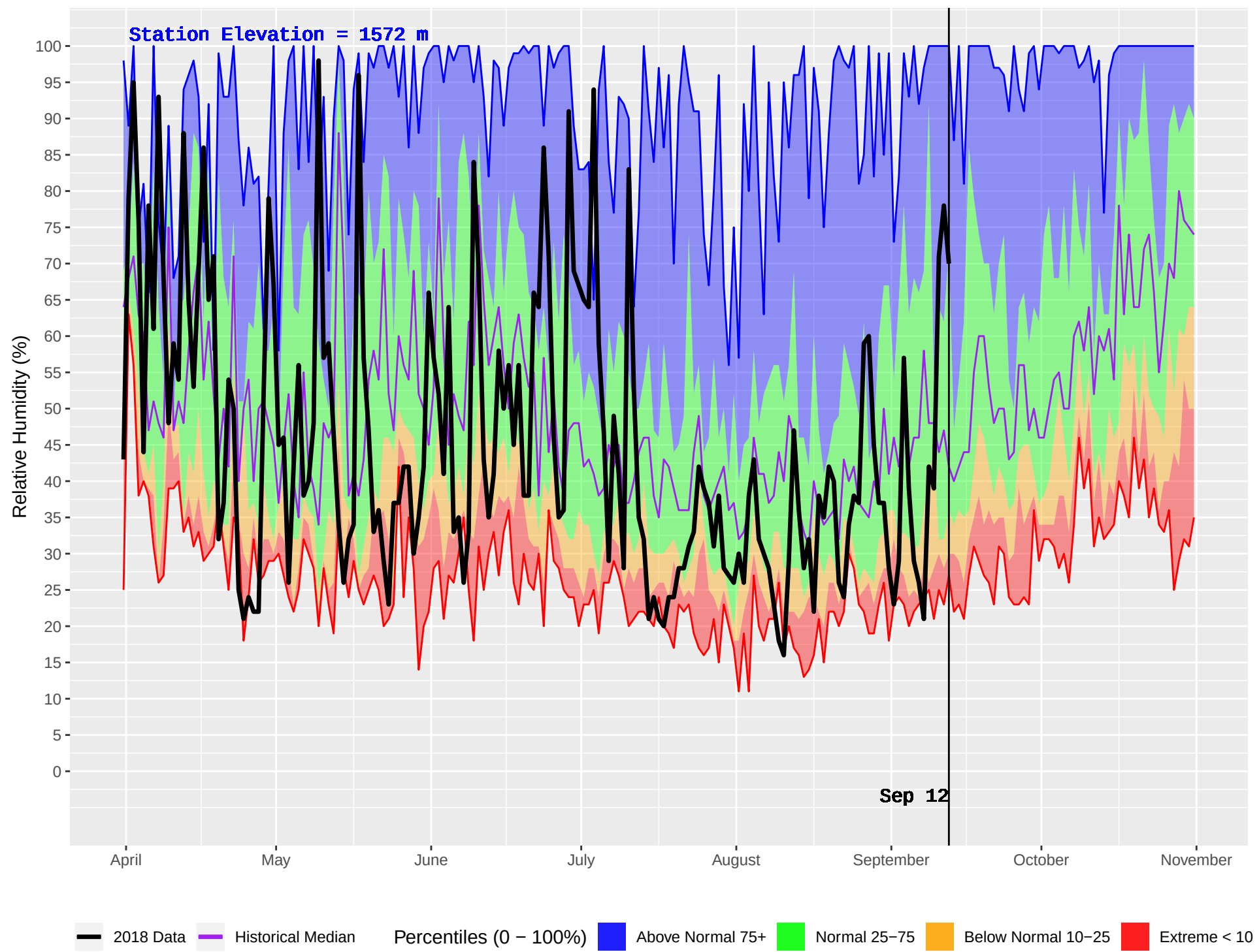
NEGRO CREEK (789) : Historical (2001–2016) and Current (2018) Daily Relative Humidity
