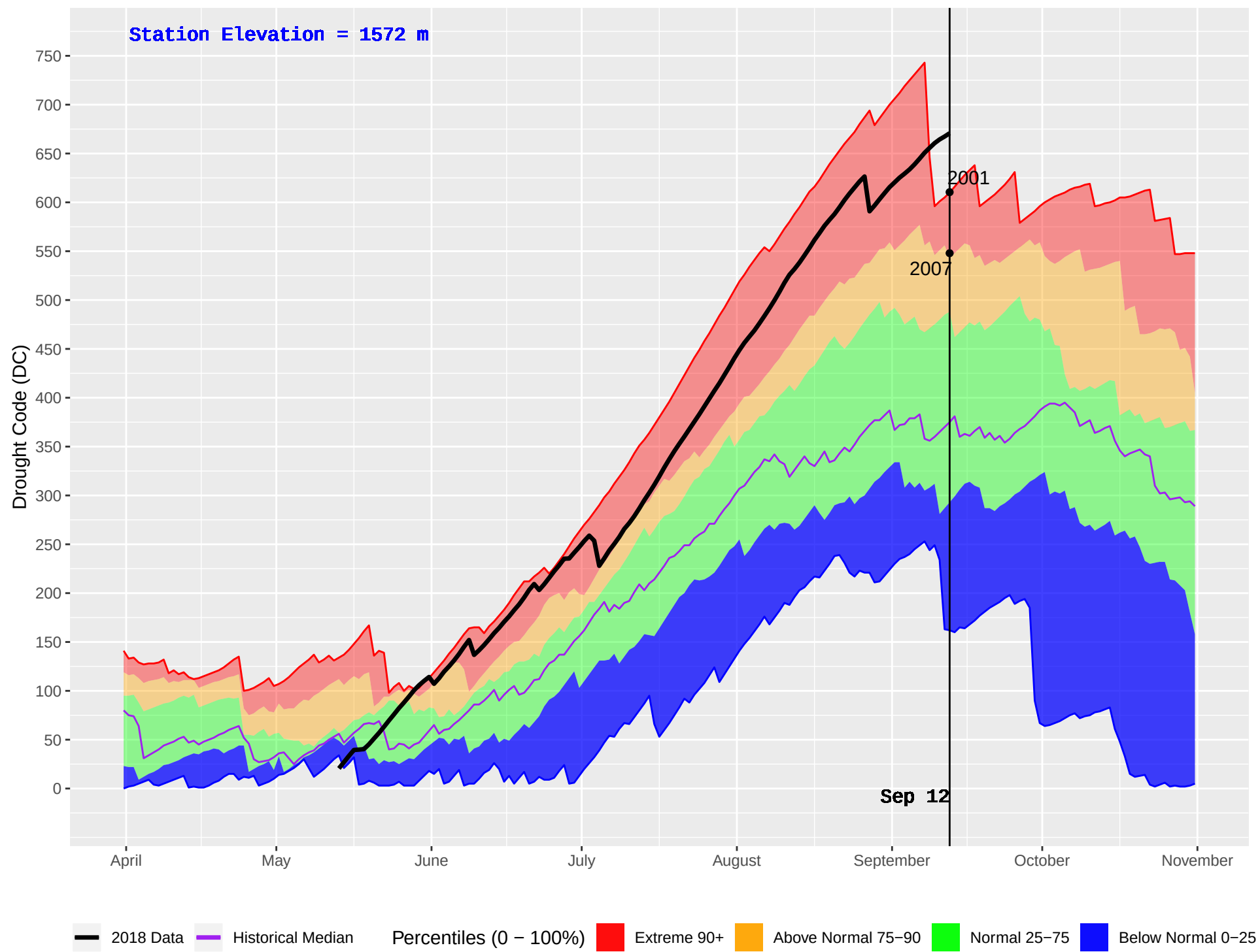
NEGRO CREEK (789) : Historical (2001–2016) and Current (2018) Daily Drought Code (DC)
